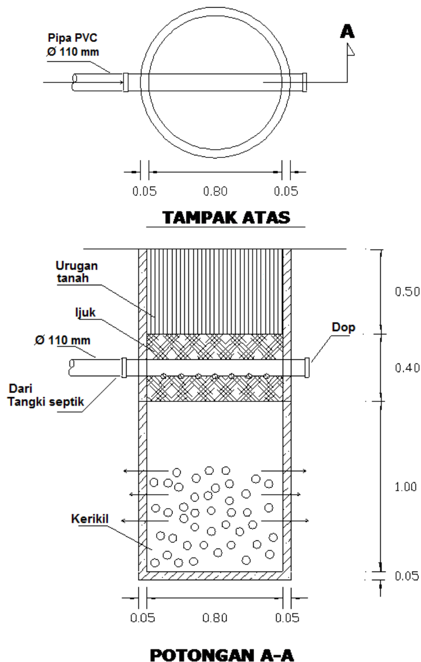
Gambar 6 – Sumur resapan
