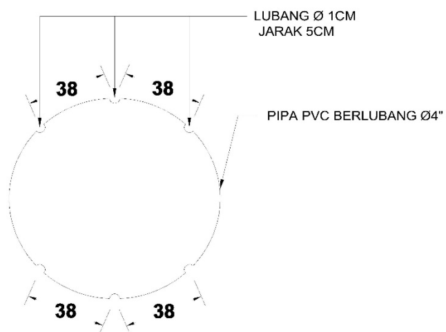
DETAIL PIPA BERLUBANG
