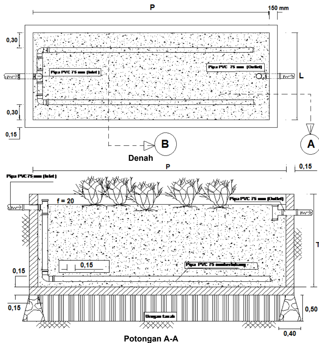
Gambar 8 – Kolam sanita
