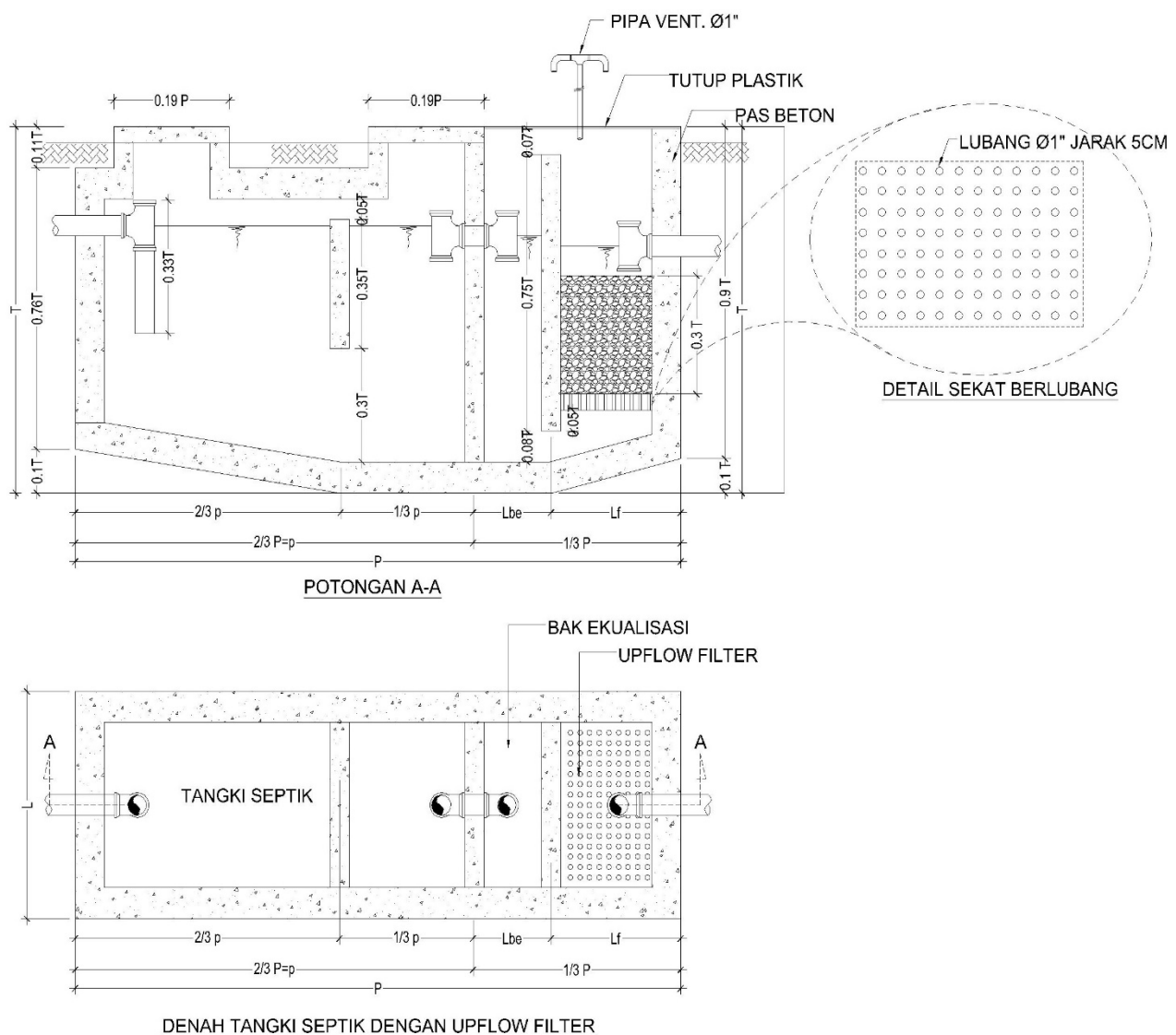
Gambar 7 – Upflow filter
